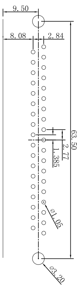
PCB layout
